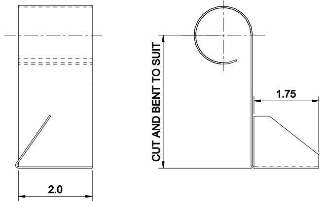
ICE DAM 20GA GALVANIZED SHT. METAL
